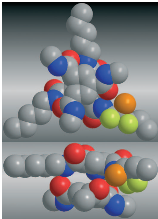
Figure 7. CPK models of aBTAs with a substituent at the 1 and 3 positions ( R configuration) highlighted in yellow and at the 2 position ( S configuration) highlighted in orange.
