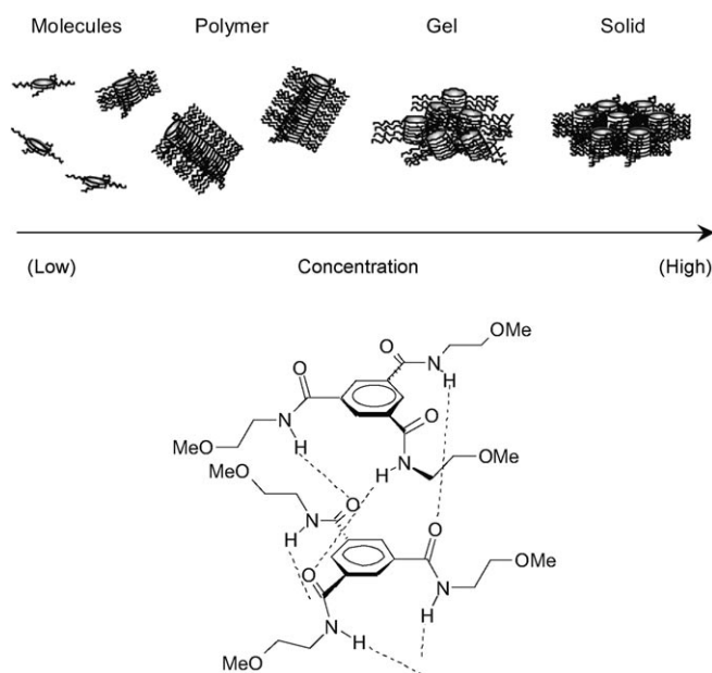
Figure 1. Different aggregation states of BTAs as function of concentration (top) and the helical packing of a BTA derivative in the solid state (bottom).
