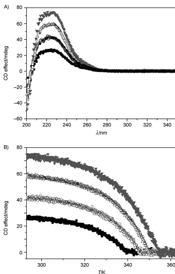
Figure 5. A) CD spectra of aBTA-R-1Me at 19 ( \blacksquare ), 30 ( \circ ), 44 ( \triangle ) and 49 \mu M ( \blacktriangledown ) at 20°C. B) Results of the temperature-dependent CD measurements of aBTA-R-1Me at 19 ( \blacksquare ), 30 ( \circ ), 44 ( \triangle ) and 49 \mu M ( \blacktriangledown ) in MCH monitored at \lambda=223 nm.
