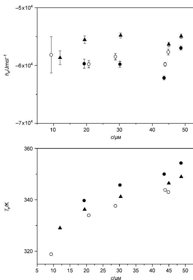
Figure 6. A) h_e as a function of concentration and B) T_c as a function of concentration, the standard deviations given for h_e result from the fit of the van der Schoot model. No standard deviations are displayed for the T_c because they are too small (typically \pm 0.05 K). ●: aBTA-R-1Me, ○: aBTA-R-3Me and ▲: aBTA-S-2Me.
