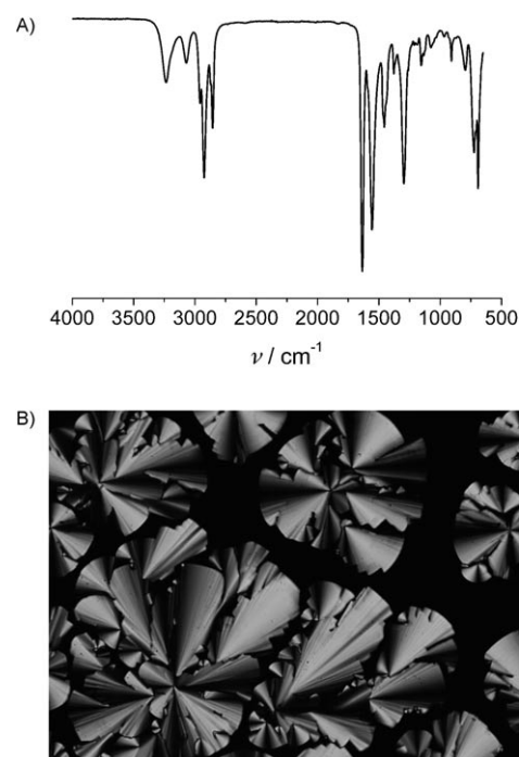
Figure 2. A) IR spectrum of aBTA- S -1Me. B) Optical texture of aBTA- R -1Me at 217^\circ\text{C} (crossed polarizers) after slow cooling from the isotropic state.
