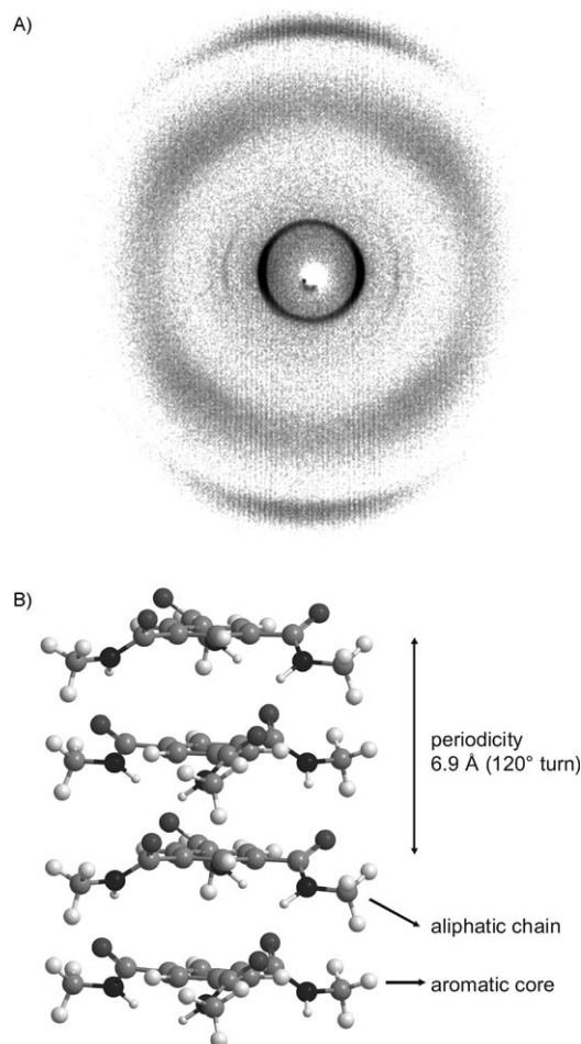
Figure 3. A) Diffraction pattern observed for aligned sBTA-C 8 measured at 159 °C. B) Model showing the proposed structure of a stack based on references [6a,b] and the characteristics of the structure, which can produce the splitting in the halo in the diffraction pattern.
