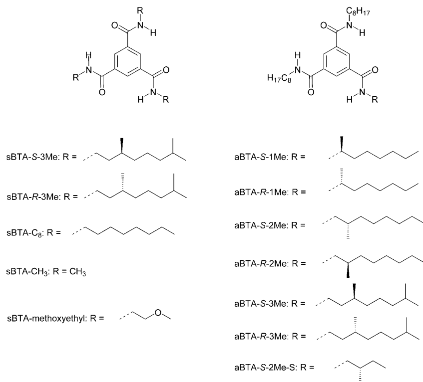
Scheme 1. Chemical structure of symmetric and asymmetric benzene-1,3,5-tricarboxamides (sBTA and aBTA, respectively).
