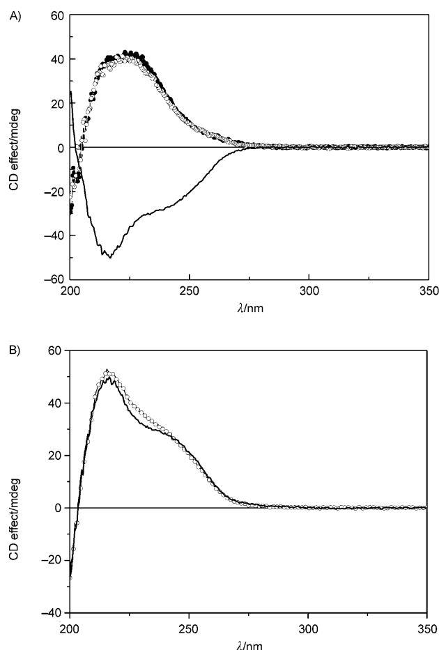
Figure 4. A) CD spectra of aBTA-R-1Me (●), aBTA-R-2Me (—) and aBTA-R-3Me (○) at a concentration of 30 \mu M in MCH at 20 °C. B) CD spectra of aBTA-S-2Me (—) at a concentration of 30 \mu M and aBTA-S-2MeBu (○) at a concentration of 140 \mu M in MCH at 20 °C.
